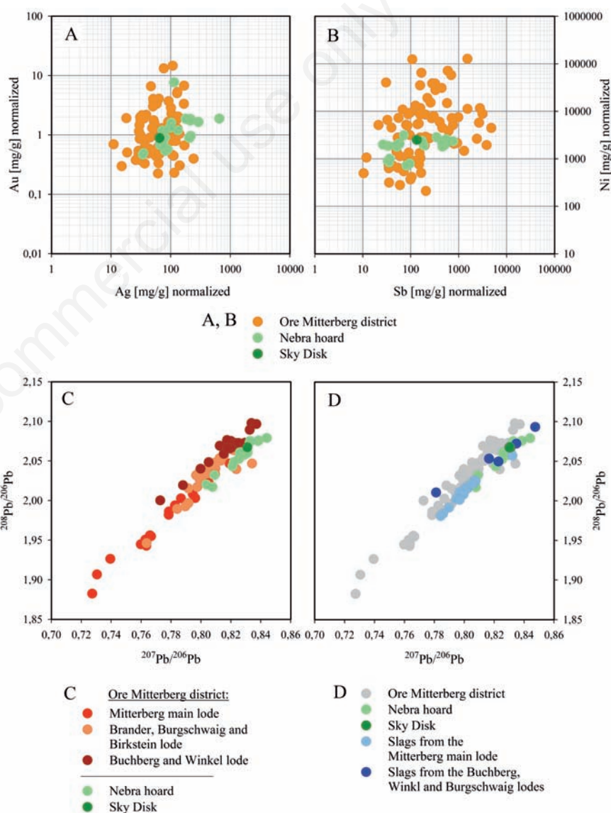
Figure 5. A,B) Trace elements in ores from the Mitterberg district and in findings from the Nebra hoard; C,D) lead isotope ratios in ores and prehistoric slags from the Mitterberg district compared with the Nebra hoard and the Sky Disk of Nebra.
