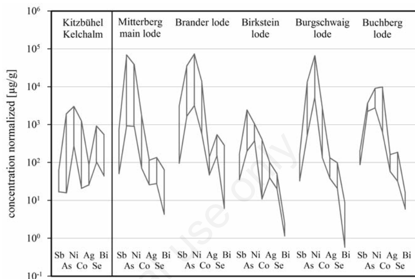
Figure 3. Trace element patterns in ores from the Kelchalm deposit and from the Mitterberg district (several different veins). The spread for some elements (Sb-As-Ni-Co-Ag-Se-Bi) is plotted on the Y-axis in the same order. The trace element signature of the Kelchalm deposit is clearly different from the Mitterberg veins.
