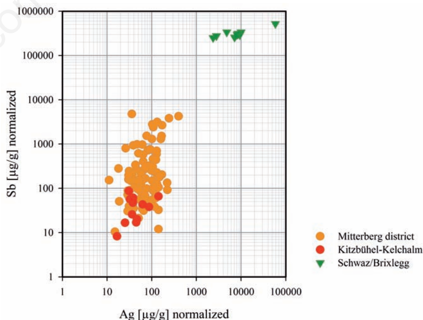
Figure 2. Ag/Sb-diagram of ores from the Mitterberg district, Kitzbühl-Kelchalm and Schwaz/Brixlegg. The fahlores from Schwaz/Brixlegg have always high concentrations of silver and antimony and can easily be distinguished geochemically.
