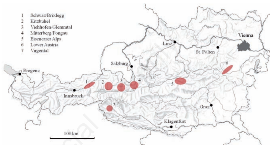
Figure 1. Prehistoric mining districts in the Eastern Alps.
